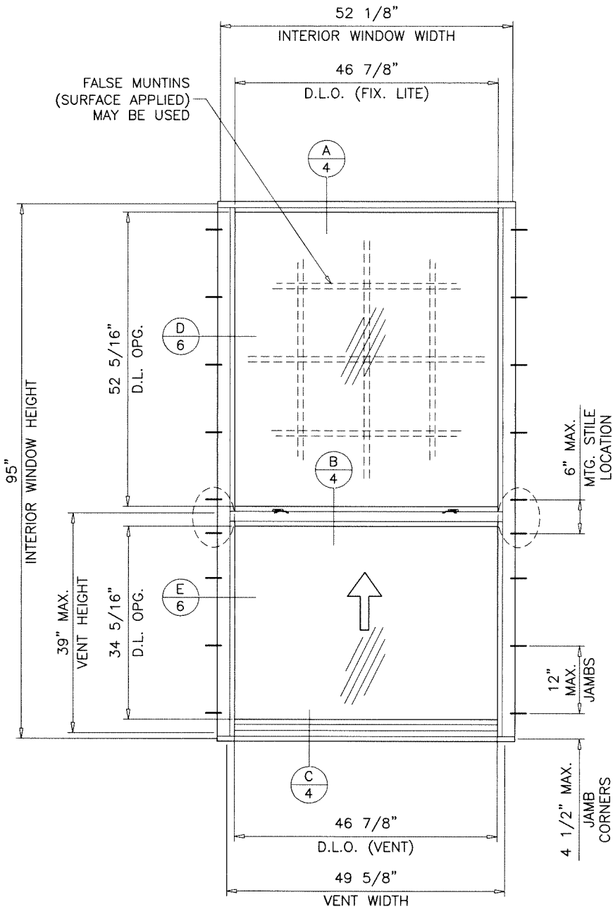
TYPICAL ELEVATION UNEQUAL LITES (ORIENTAL TYPE) TESTED UNIT
